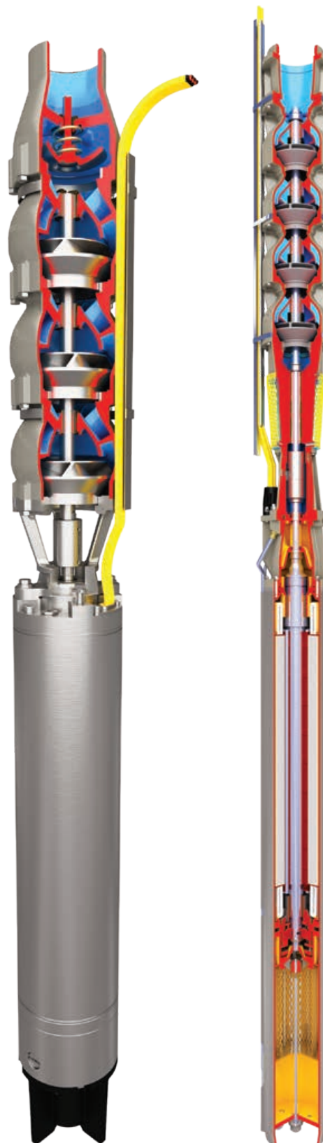
SUBM pump with H2O motor
