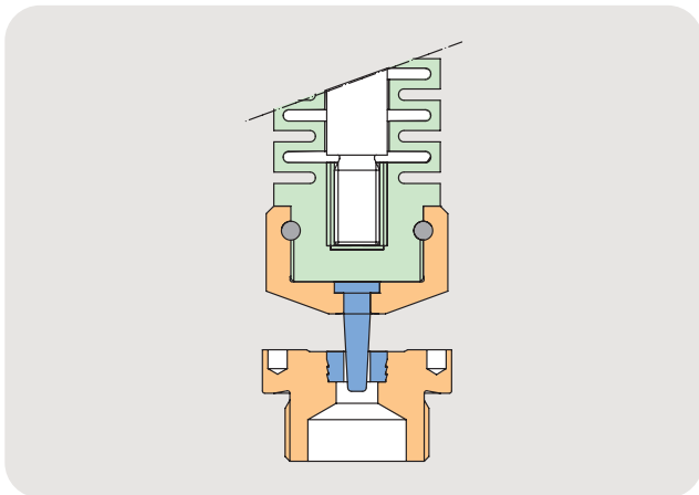
Hastelloy Plug and Seat Inserts
