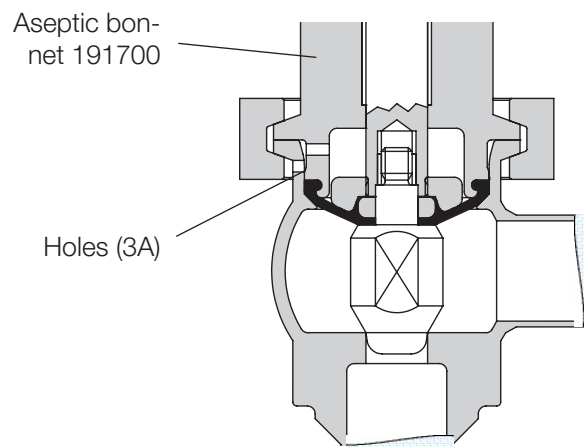
Figure 6: Type 191700 3A design
