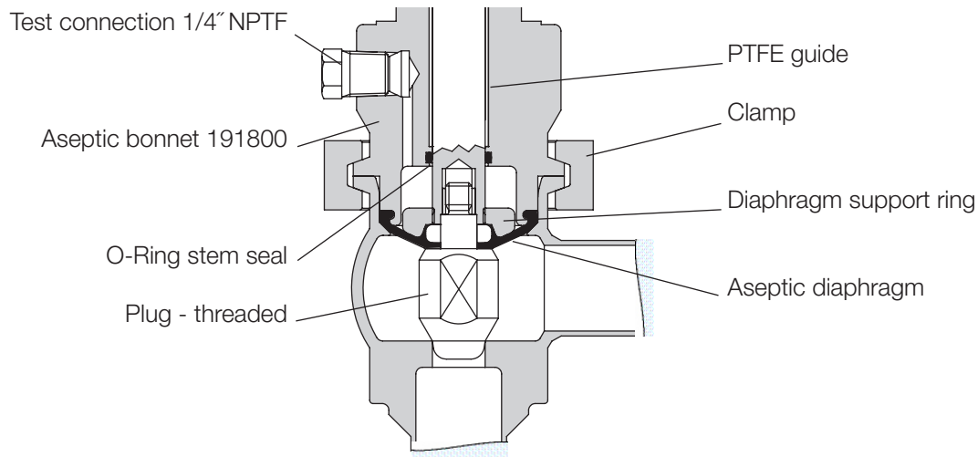
Figure 7: Type 191800 with test port connection
