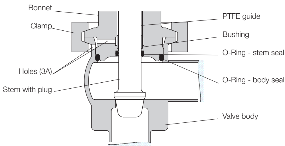
Figure 7: Type 191800 with test port connection
