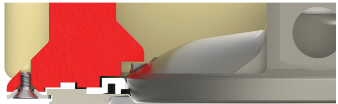
Figure 6: Dual fire-safe seating arrangement
