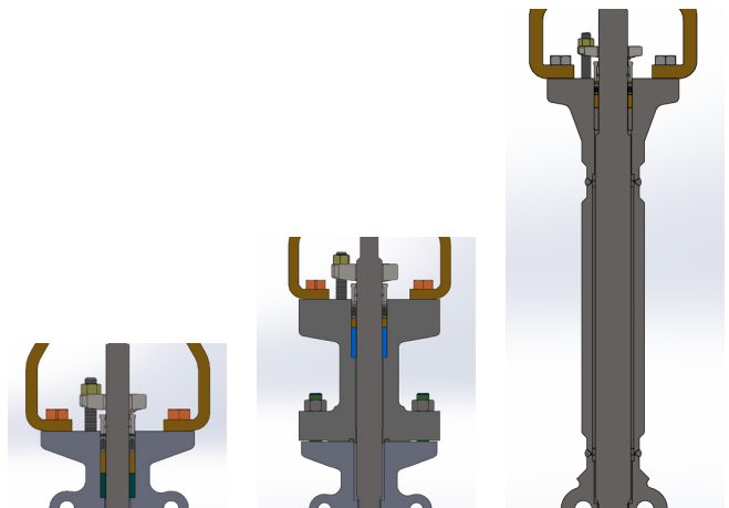
Figure 7: Standard bonnet
