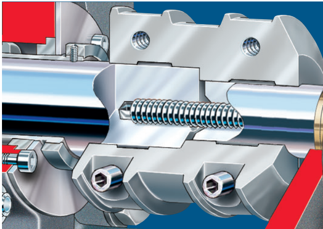
Investment cast (WEB) muff coupling
