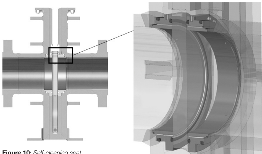
Figure 10: Self-cleaning seat
