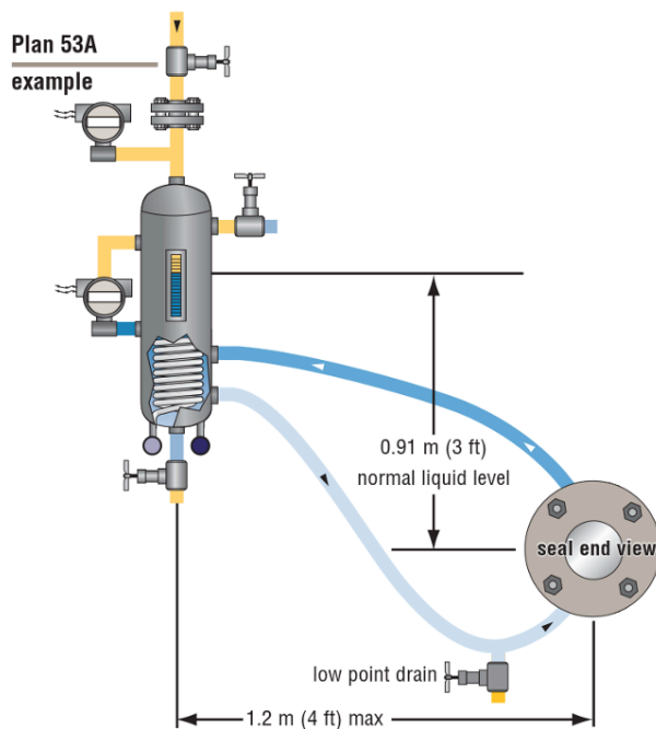
Figure 7: Piping Plan 53A mounting dimensions example
