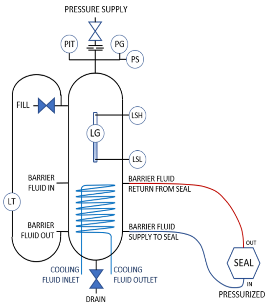
Figure 4: Recommended P&ID piping plan 53A
