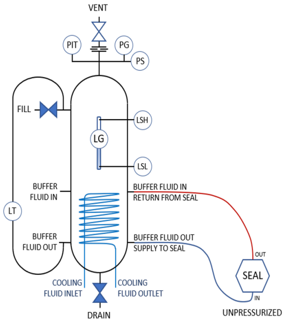
Figure 3: Recommended P&ID piping plan 52
