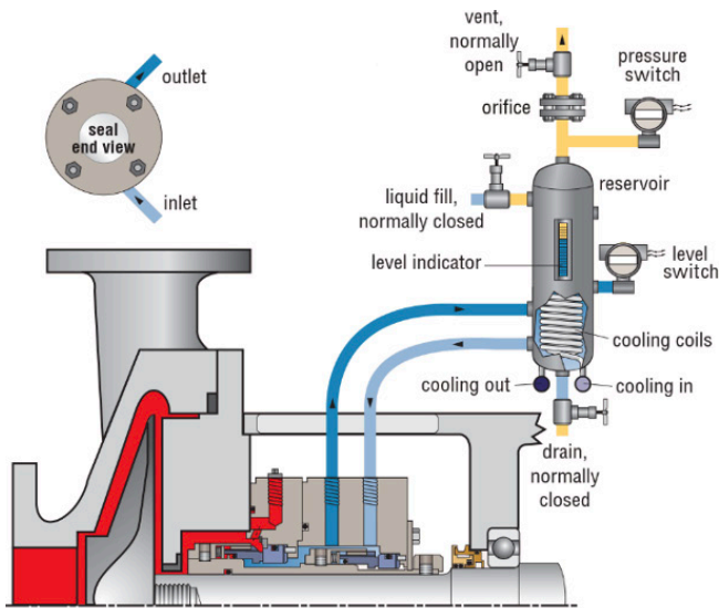
Figure 5: Piping Plan 52 configuration
