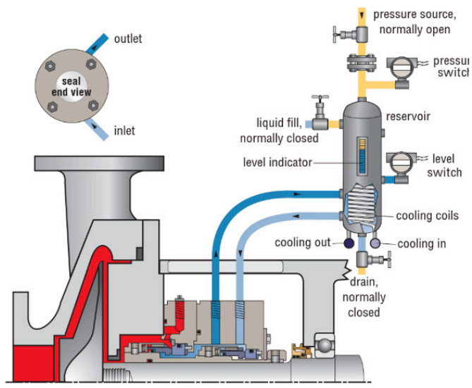
Figure 6: Piping Plan 53A configuration
