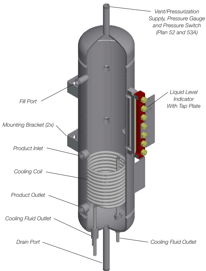
Figure 1: 682R51 Reservoir sectional view
