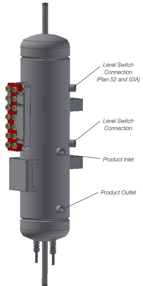
Figure 2: 682R51 external view
