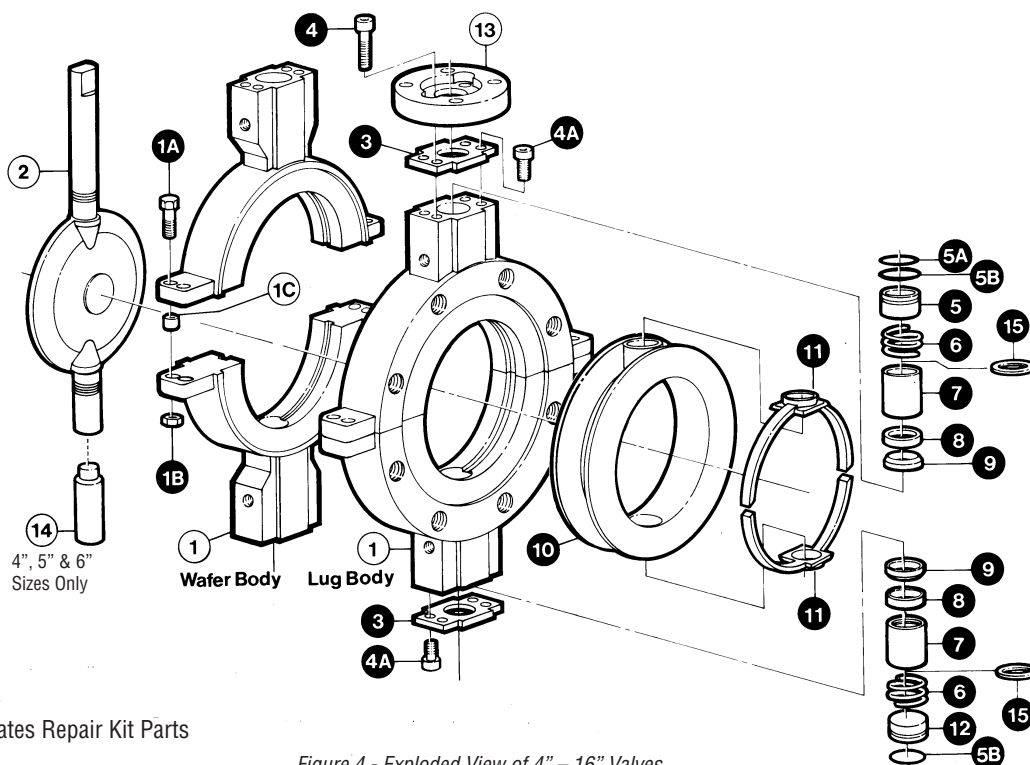
Figure 4 - Exploded View of 4" – 16" Valves
