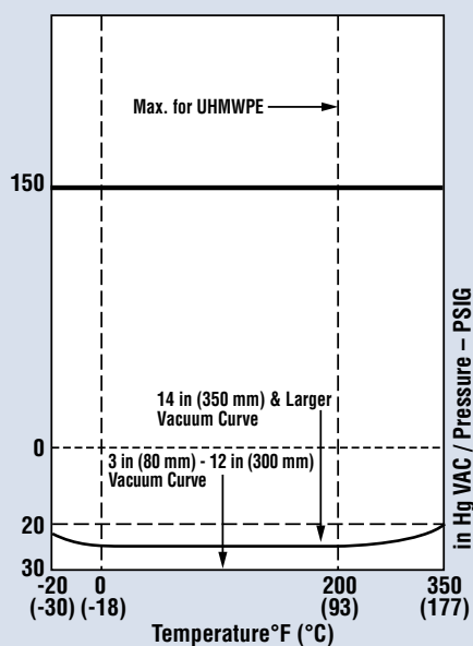
Pressure-Temperature Curve
