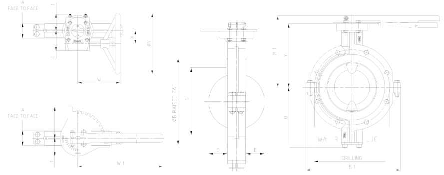
Dimensions for BTV-2000 Wafer and Lug Valves With Gear Operators
