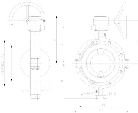
Dimensions for BTV-2000 Wafer and Lug Valves With Gear Operators
