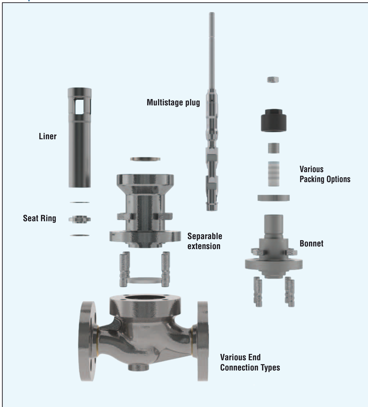
Figure 5: Exploded View
