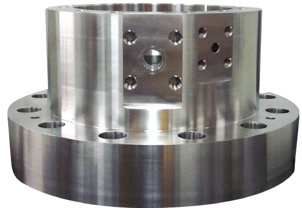
First-stage seal housing with integral flanges.
