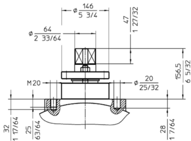
FK76C Topwork drawing 3Z2102
