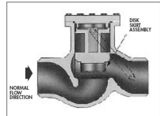
Figure 1: Globe Check Valve with Fabricated Disk Skirt.
