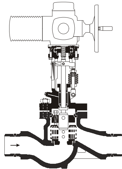
Control valve ZK 29/14 DN 80 with rotary actuator, butt-weld ends, sealing-fluid connection and self-tightening stuffing box (special equipment)
